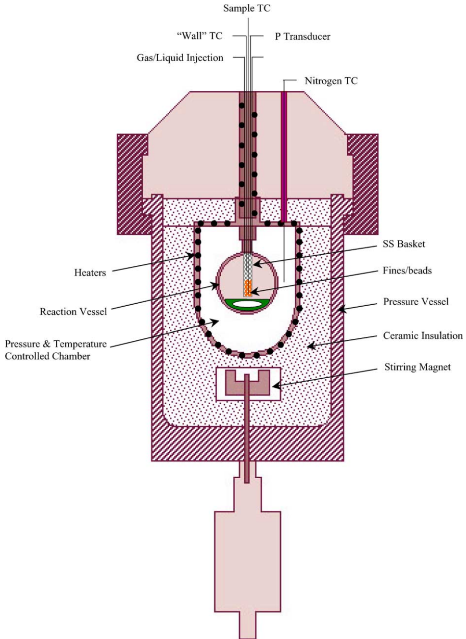
Fig. 1. Depiction of the Automatic Pressure Tracking Adiabatic Calorimeter (APTAC™).
