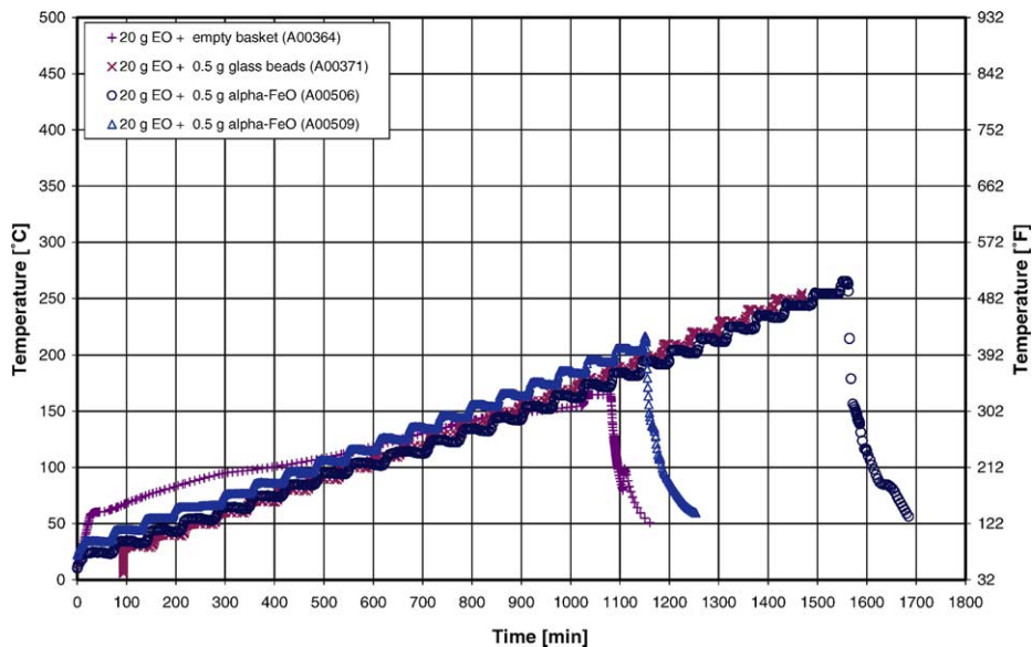
Fig. 2. Temperature history of ethylene oxide in contact with glass and \alpha -FeO in the APTAC™.
