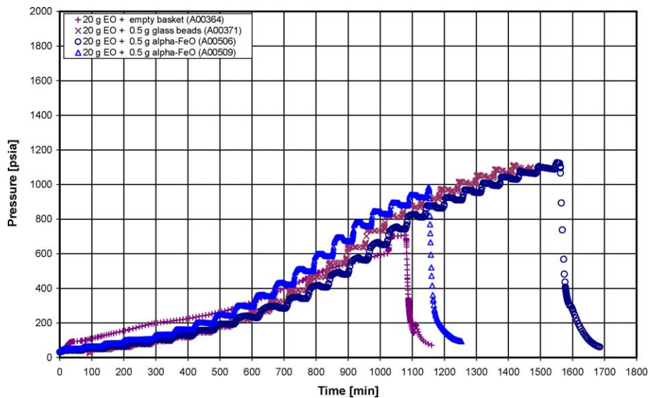
Fig. 3. Pressure history of ethylene oxide in contact with glass and \alpha -FeO in the APTAC™.
