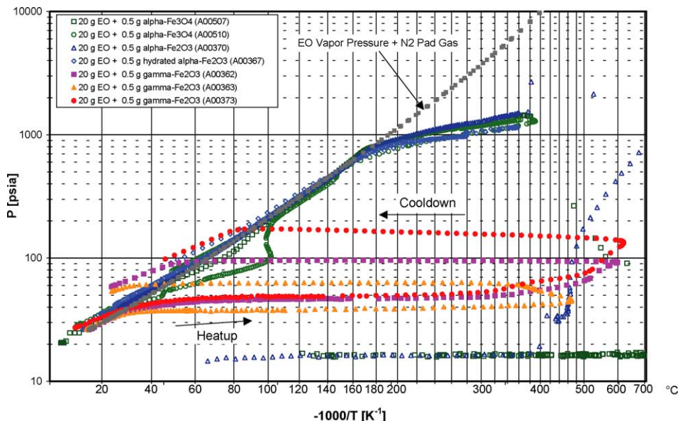
Fig. 14. Pressure–temperature profiles of ethylene oxide in contact with iron oxide in the APTAC™.
