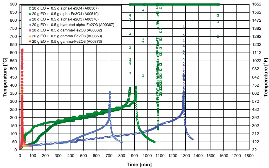
Fig. 8. Temperature history of ethylene oxide in contact with iron oxide in the APTAC™.
