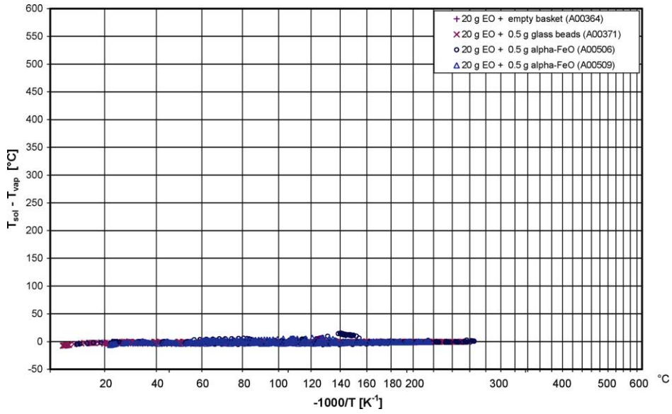
Fig. 4. Temperature difference between solid and gas phase of ethylene oxide in contact with glass and \alpha -FeO in the APTAC TM .
