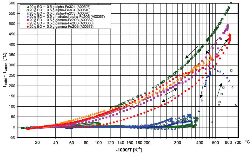
Fig. 10. Temperature difference between solid and vapor phases of ethylene oxide in contact with iron oxide in the APTAC™.
