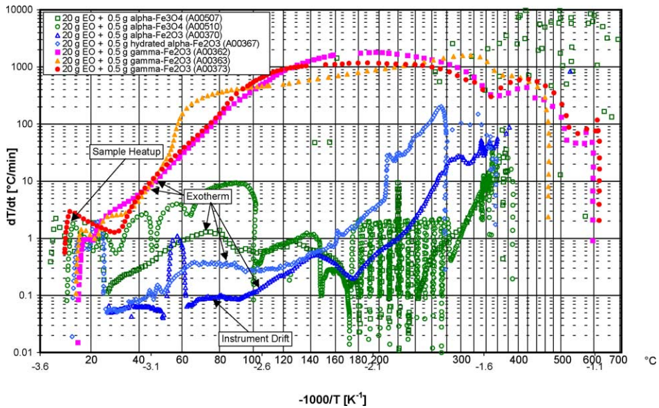
Fig. 11. Self-heat rate profiles of ethylene oxide in contact with iron oxide in the APTAC™.
