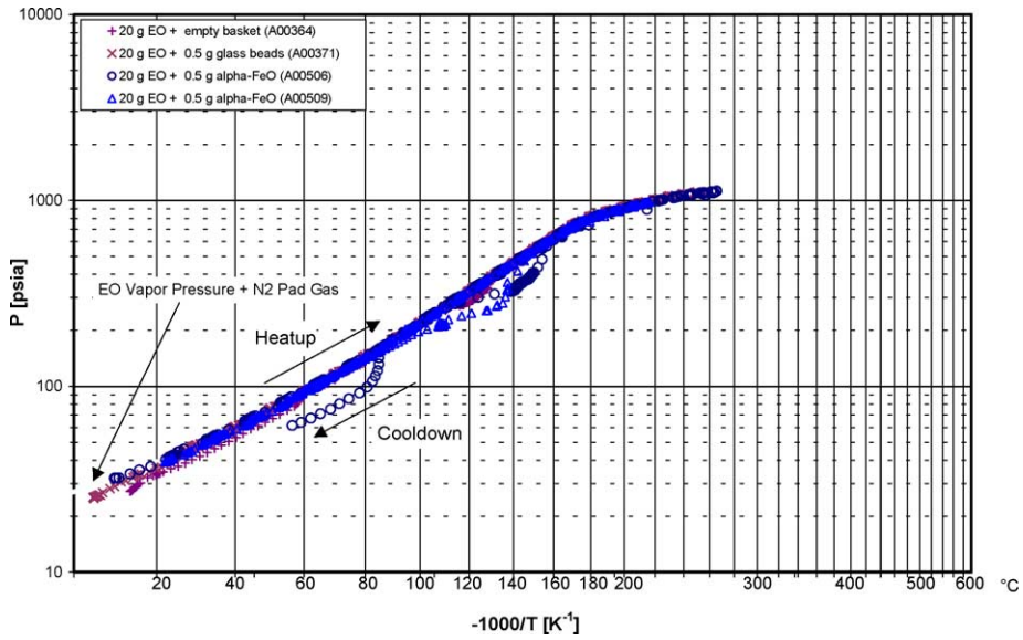
Fig. 7. Pressure–temperature profiles of ethylene oxide in contact with glass and \alpha -FeO in the APTAC™.
