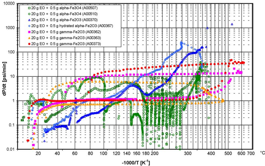
Fig. 13. Pressurization rate profiles of ethylene oxide in contact with iron oxide in the APTAC™.
