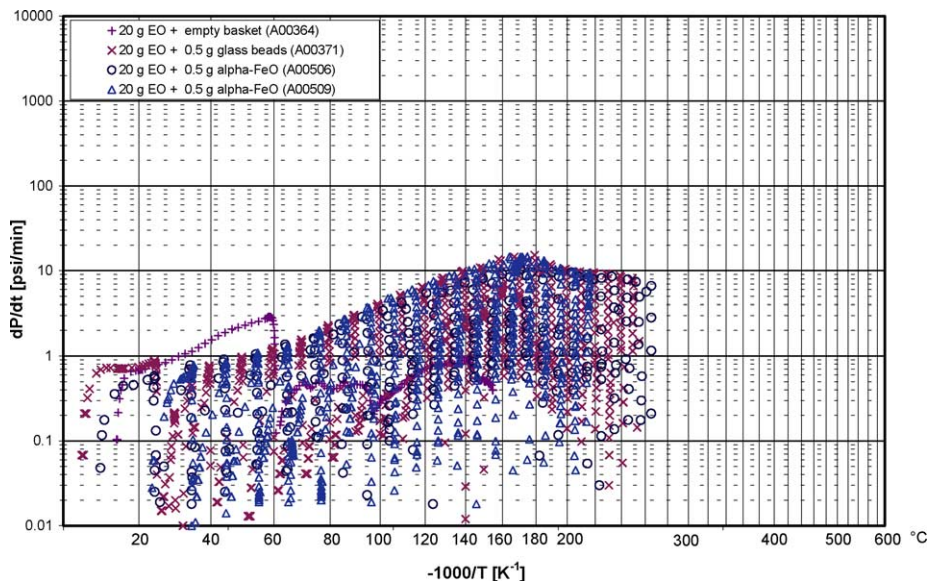
Fig. 6. Pressurization rate profiles of ethylene oxide in contact with glass and \alpha -FeO in the APTAC TM .
