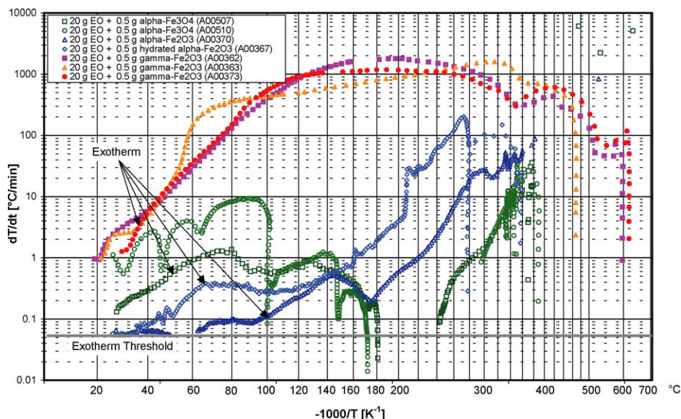
Fig. 12. Self-heat rate profiles of ethylene oxide in contact with iron oxide in the APTAC TM ; heat-wait-search steps removed.
