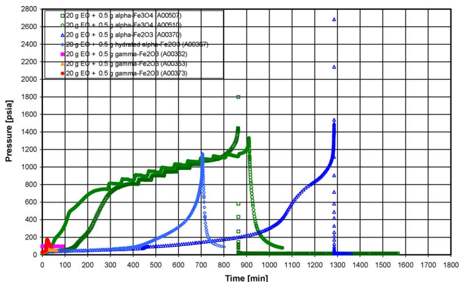
Fig. 9. Pressure history of ethylene oxide in contact with iron oxide in the APTAC™.
