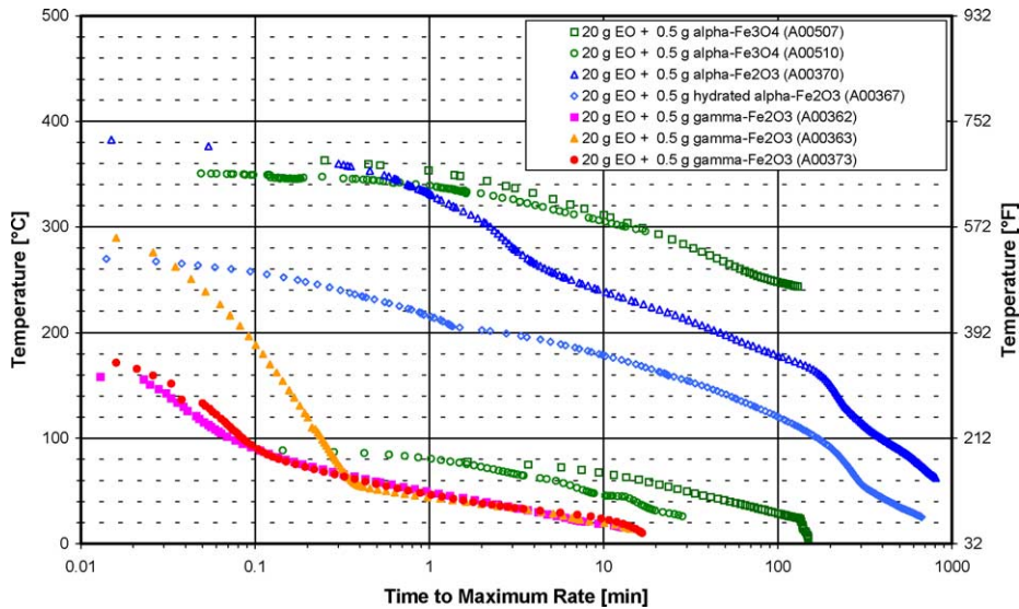
Fig. 15. Time-to-maximum rate profiles of ethylene oxide in contact with iron oxide in the APTAC™.
