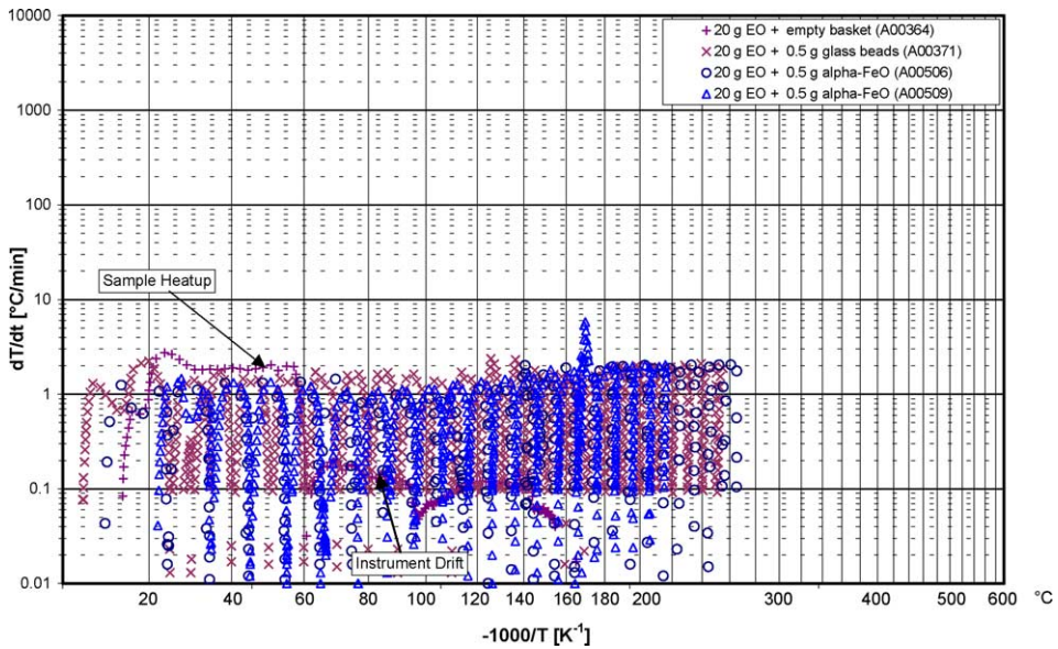
Fig. 5. Self-heat rate profiles of ethylene oxide in contact with glass and \alpha -FeO in the APTAC TM .
